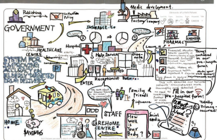
Rich Picture
